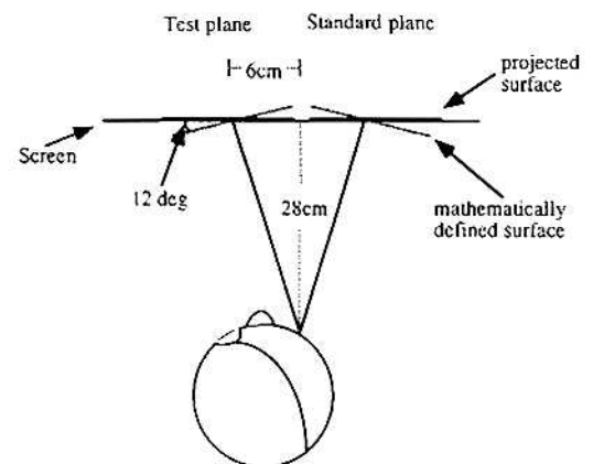
Fig. 2. Top view of the experimental setup.
