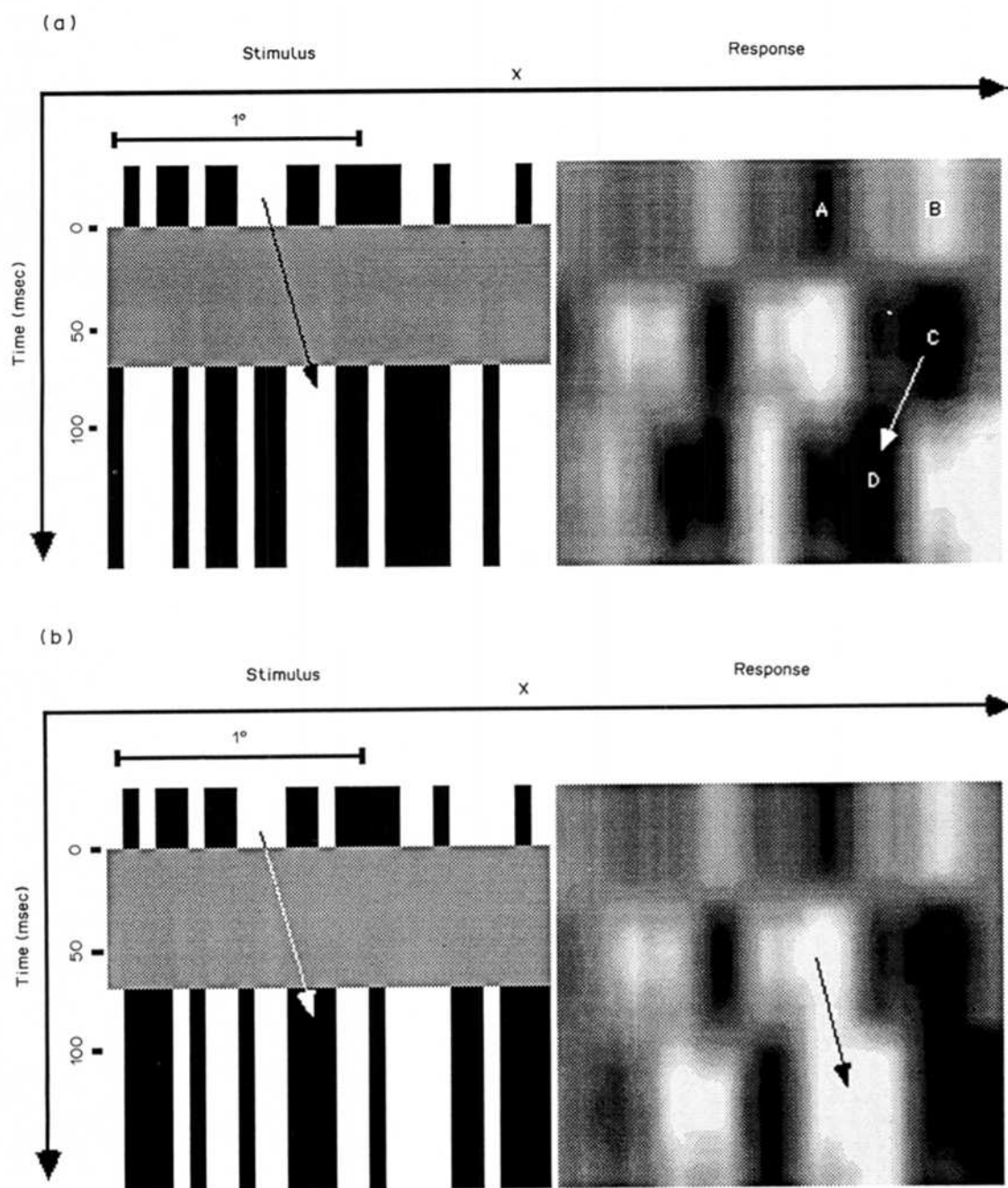
Fig. 6. Temporal responses predicted from equation (1) for the displacement of a row in a random-dot field. Stimulus is shown in the left of each response image. x -axis show horizontal position in space and y -axis shows time with respect to the onset of the ISI field. The same pattern is displaced 0.19 deg to rightward: (a) 70 msec ISI with a grey field for a normal kinematogram; (b) 70 msec ISI with a grey field for a contrast-reversed kinematogram. Arrows indicate physical displacement on the left and energy displacement in filtered image on the right.
