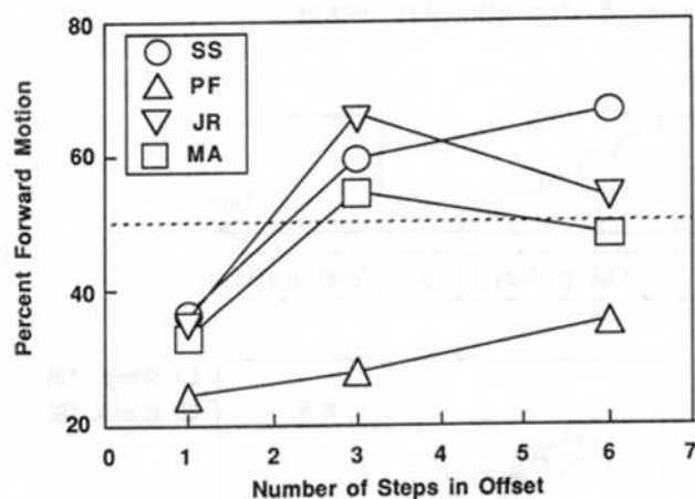
Fig. 5. Percentage of responses for the direction of displacement as a function of offset-step number, provided by pooling data for ISIs between 17 and 67 msec from Figs 1 and 4. Difference symbols represent different observers. The broken line shows chance level of response.
